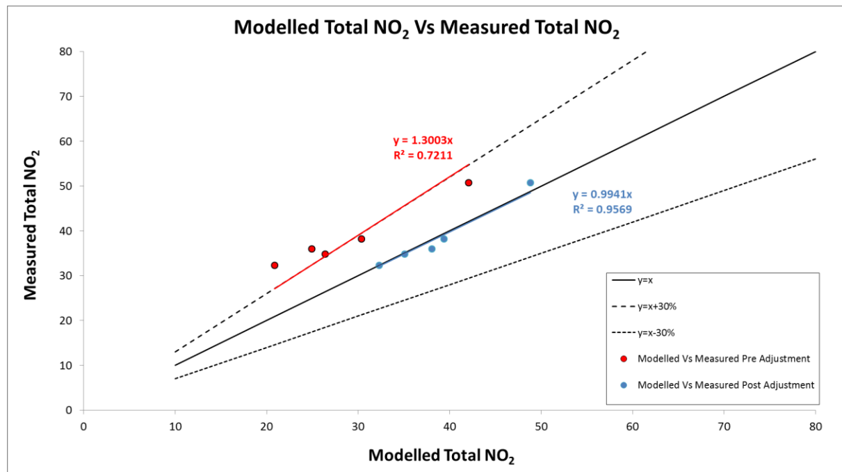
Figure 3: Linear regression analysis of modelled vs. monitored NO 2 annual mean 2010
